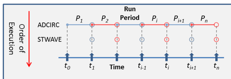
Figure 8-2. A workflow schematic showing the order of operation between ADCIRC and STWAVE within the CSTORM-MS coupling framework. Red and blue alternating patterns are used for visual effects only to show separation of individual run periods.
