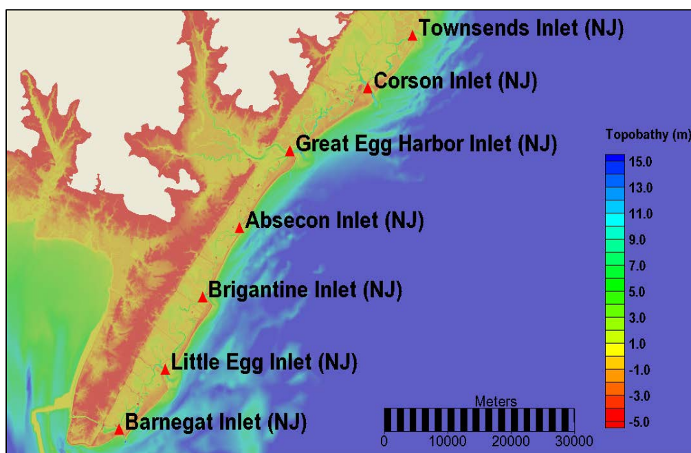
Figure 6-14. NAP save point locations at 7 inlets in New Jersey; the ADCIRC mesh resolution for these inlets ranges from 70-200 meters.
