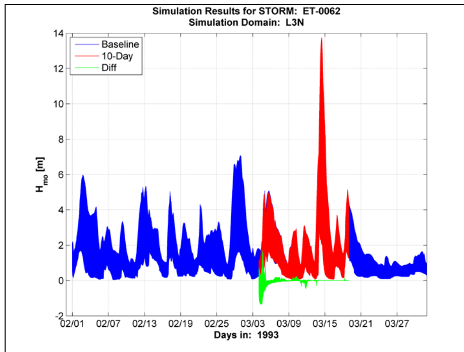
Figure 5-12. Time plot envelope of 165 special output locations for 10-day pad, Storm of the Century.
