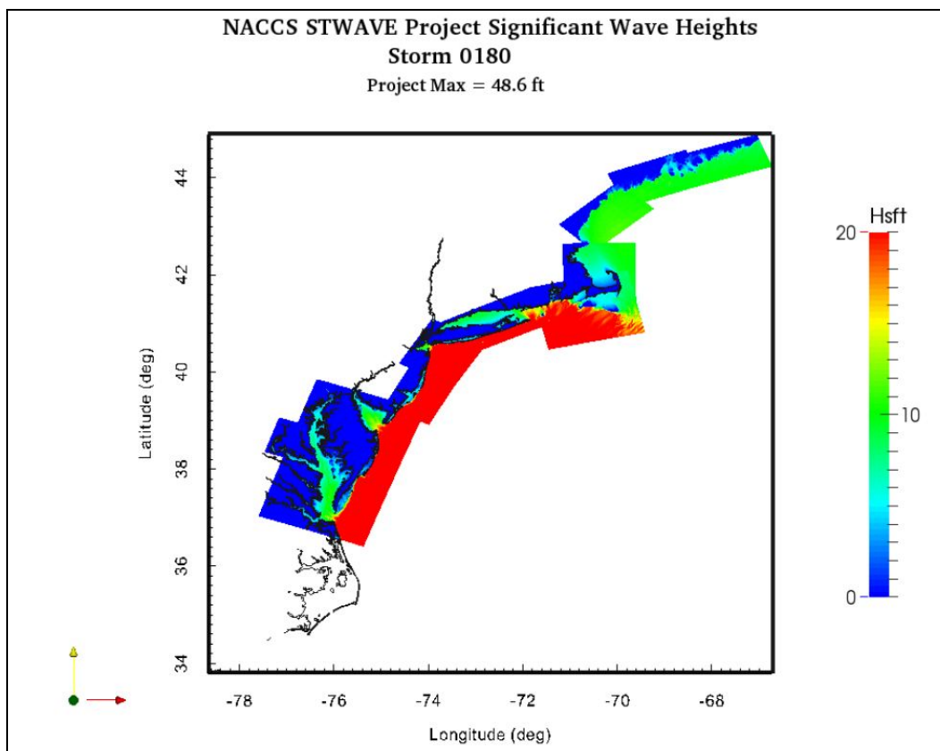
Figure 8-12. STWAVE peak wave heights combined overview contour plot for synthetic tropical storm number 180.
