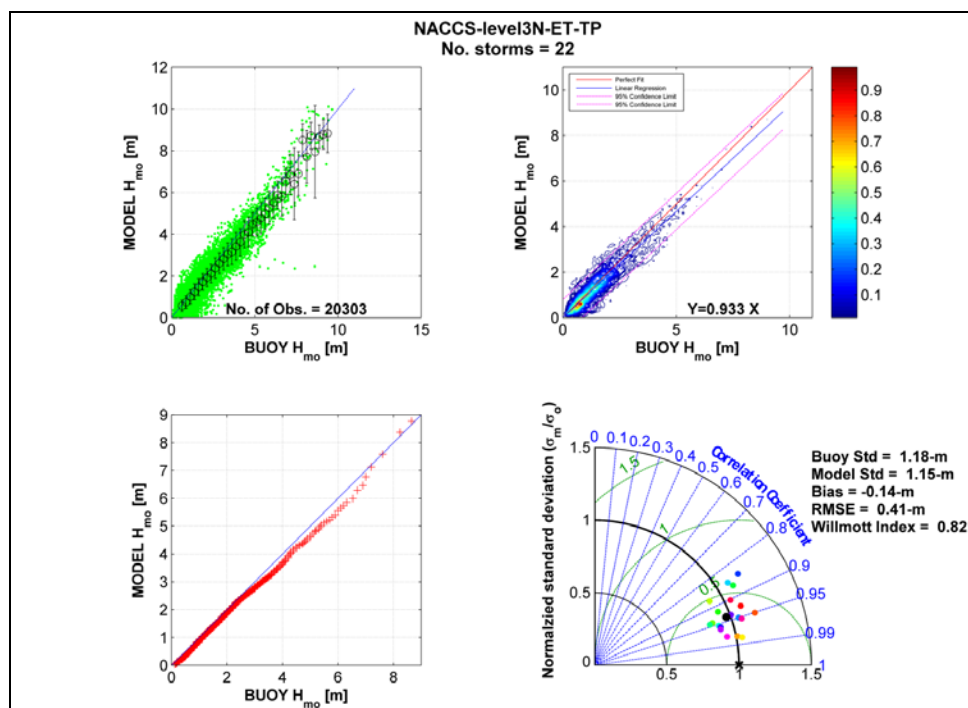
Figure 5-20. Bin average scatter diagram (top left), color contour (top right), Quartile-Quartile plot (lower left) and Taylor diagram (lower right) for WAM Level3N results derived from the extra- and tropical storm set.
