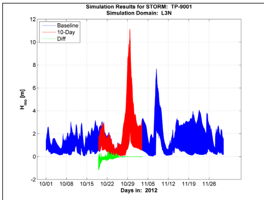
Figure 5-16. Time plot envelope of 165 special output locations for 10-day pad SuperStorm Sandy.
