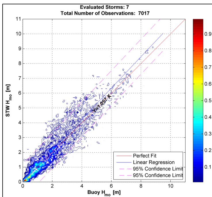
Figure 7-24. Color contour of time paired significant wave heights for all validation storms.
