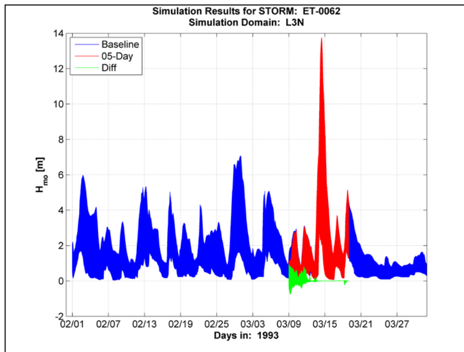
Figure 5-13. Time plot envelope of 165 special output locations for 05-day pad, Storm of the Century.
