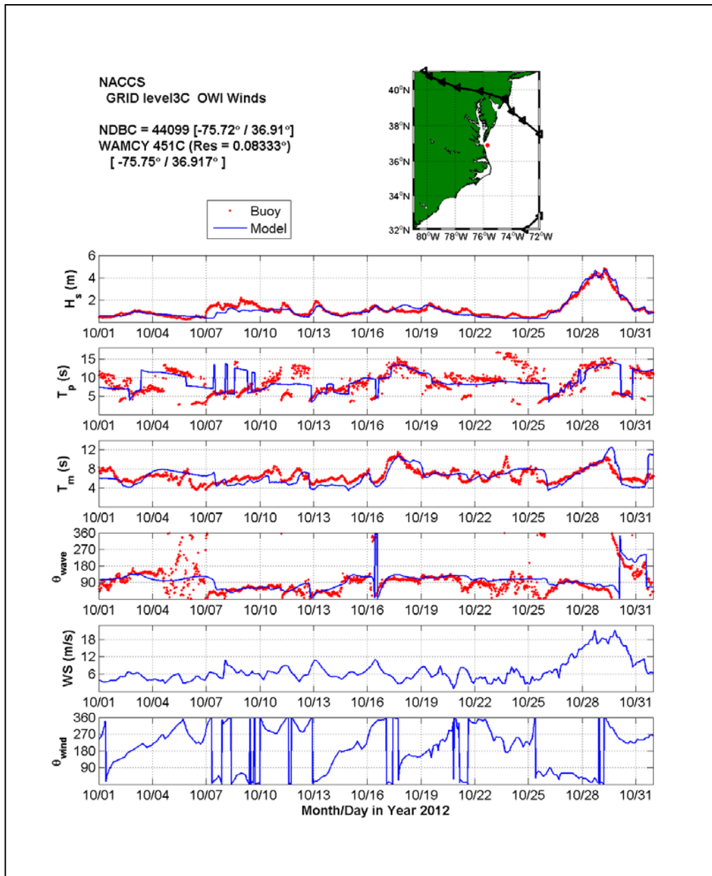
Figure 5-10. Evaluation of WAM results at NDBC 44099, the significant wave height, parabolic fit wave period, the mean wave period, and the vector mean wave direction.
