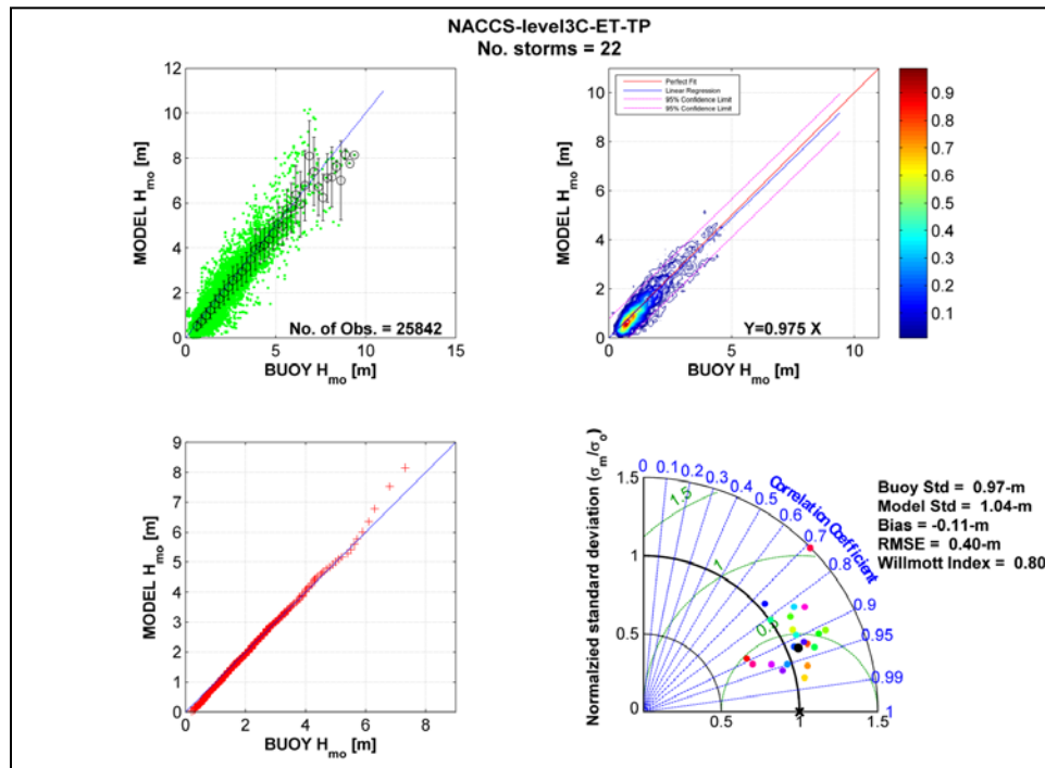
Figure 5-21. Bin average scatter diagram (top left), color contour (top right), Quartile-Quartile plot (lower left) and Taylor diagram (lower right) for WAM Level3C results derived from the extra- and tropical storm set.
