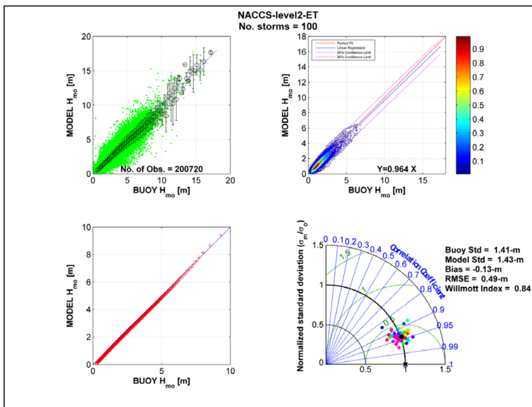
Figure 5-26. Bin average scatter diagram (top left), color contour (top right), Quartile-Quartile plot (lower left) and Taylor diagram (lower right) for WAM Level2 results derived from the 100 extreme extratropical storm events.
