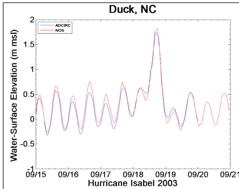
Figure 6-32. Hurricane Isabel time series comparison at Duck, North Carolina.
