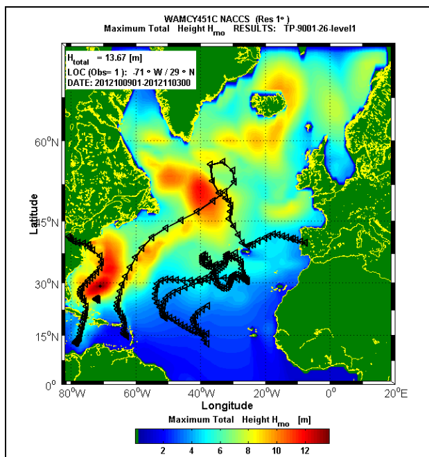
Figure 5-2. Maximum wave height envelope during SuperStorm Sandy 26-day simulation, where five tropical systems were evident in the Level 1 Atlantic Ocean domain.
