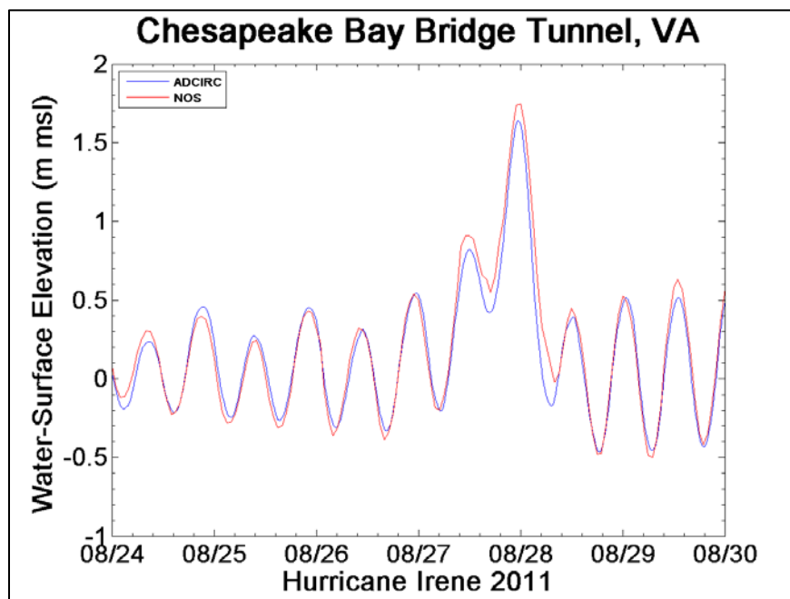
Figure 6-33. Hurricane Irene time series comparison at Chesapeake Bay Bridge Tunnel, Virginia.
