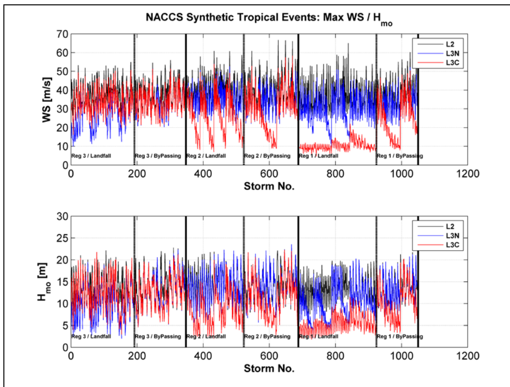
Figure 5-29. Overall maximum wind speed (top panel) and maximum significant wave height (bottom panel) estimates for each of the 1050 synthetic tropical storm simulations for the NACCS.
