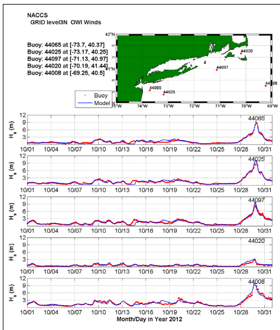
Figure 5-9. Evaluation of WAM Level3N, Long Island region results for five wave measurement locations.
