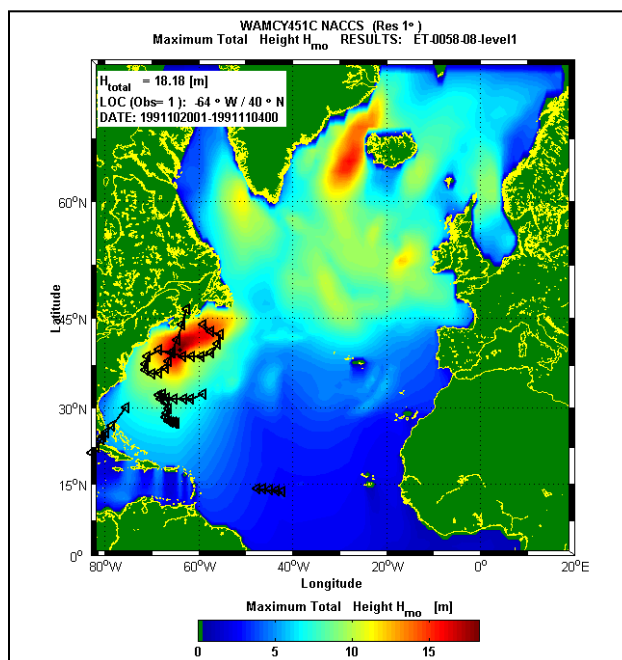
Figure 5-3. Maximum wave height envelope during Halloween Nor 'Easter (ET0058-8) 8-day simulation, where three tropical systems were evident in the Level 1 Atlantic Ocean domain.
