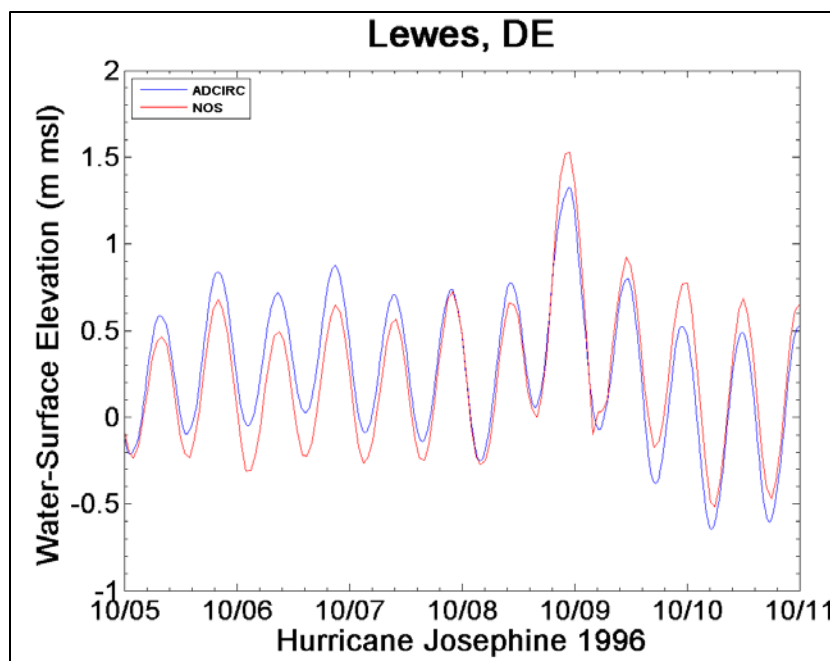
Figure 6-31. Hurricane Josephine time series comparison at Lewes, Delaware.
