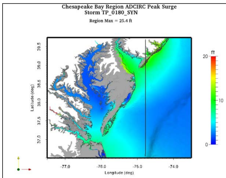
Figure 8-9. Chesapeake Bay region ADCIRC peak surge contour plot for synthetic tropical storm number 180.
