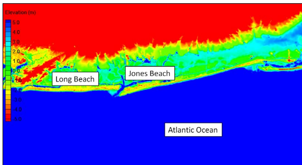
Figure 6-6. ADCIRC mesh topography/bathymetry for a portion of Long Island, New York after 2012 LIDAR update.
