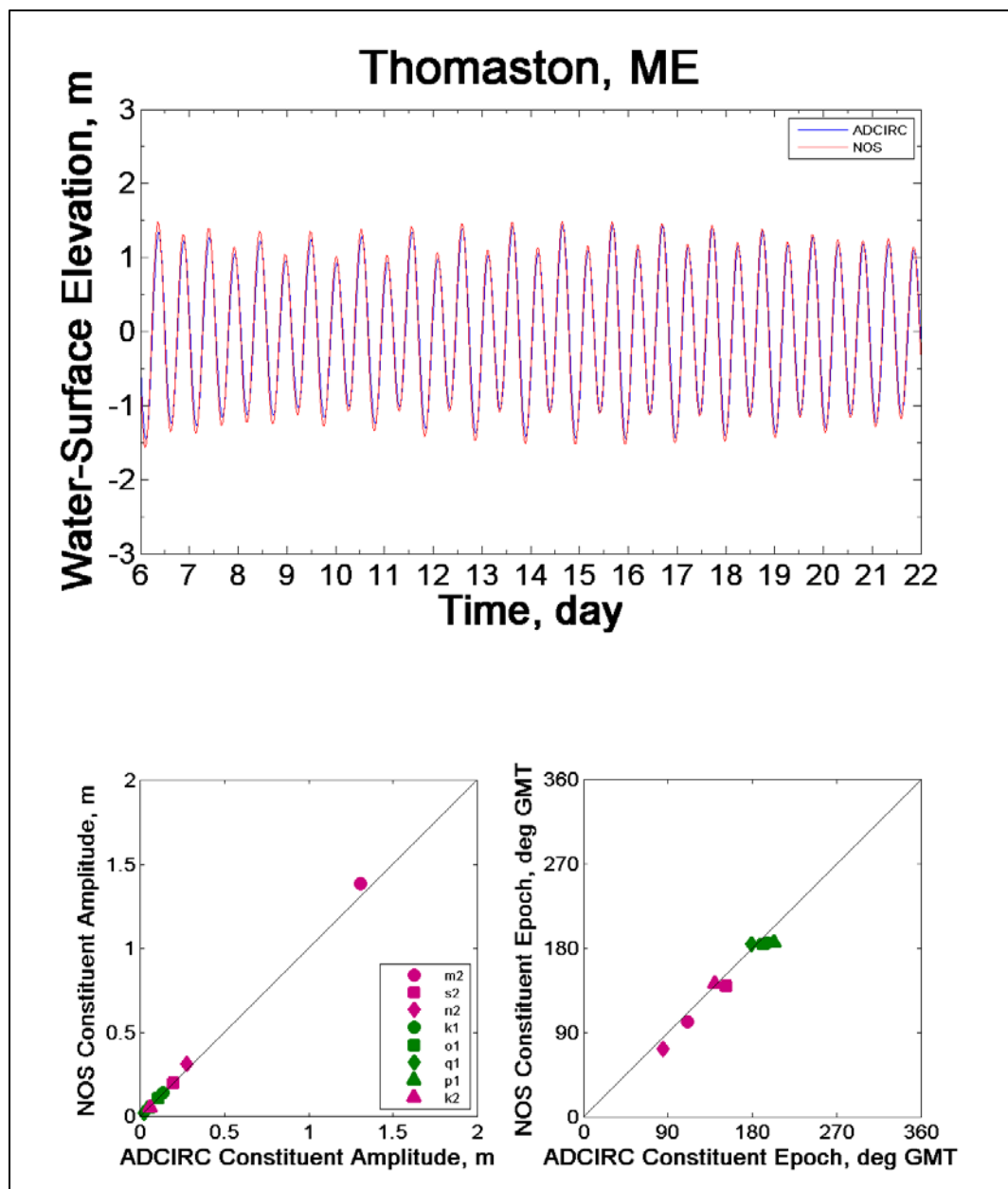
Figure 6-22. Tidal harmonic analysis for Thomaston, Maine.
