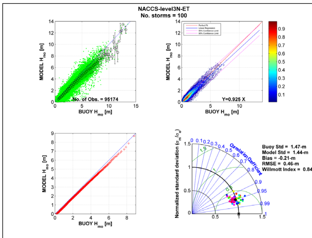
Figure 5-27. Bin average scatter diagram (top left), color contour (top right), Quartile-Quartile plot (lower left) and Taylor diagram (lower right) for WAM Level3N results derived from the 100 extreme extratropical storm events.
