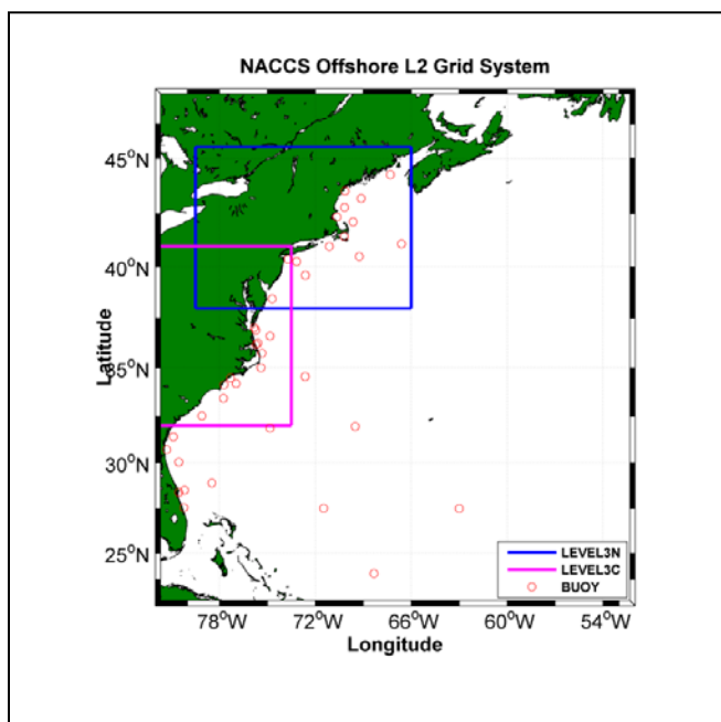
Figure 5-5. WAM multi-level grid system used in NACCS. Note Level 2 covers the entire domain illustrated.
