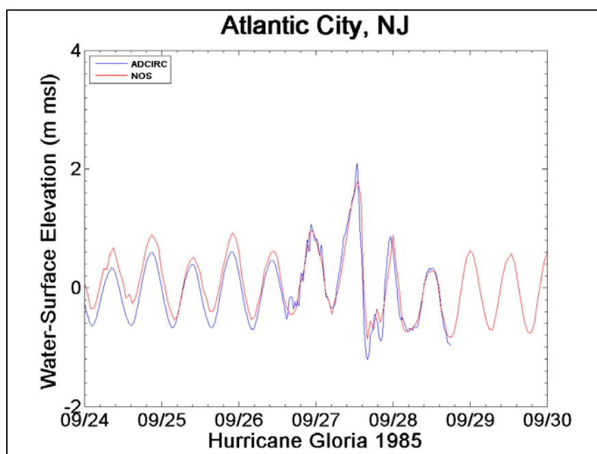
Figure 6-30. Hurricane Gloria time series comparison at Atlantic City, New Jersey.
