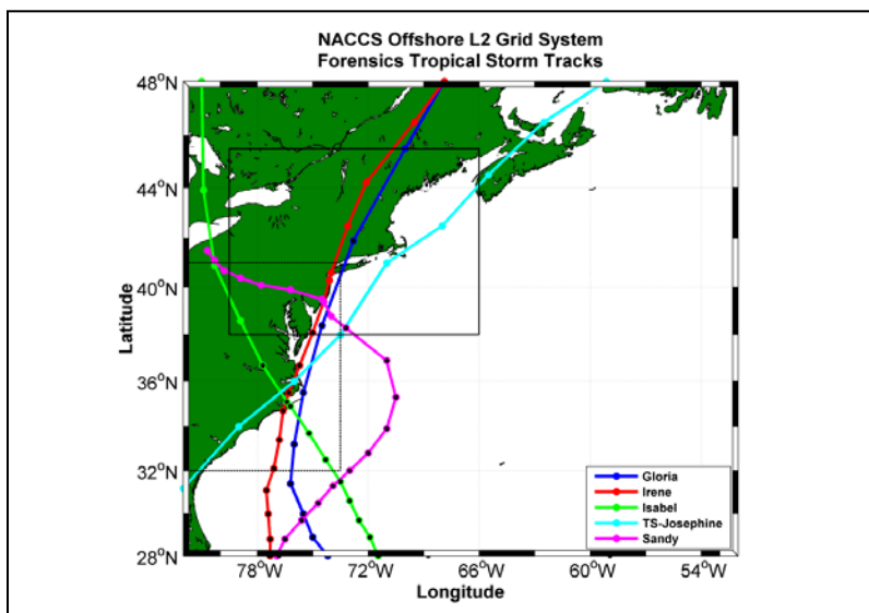
Figure 5-6. Five tropical storm tracks used in evaluation tests. Level3N and Level3C domains are identified by the black boxes, black dot represents hurricane intensities of Cat-1 and higher.
