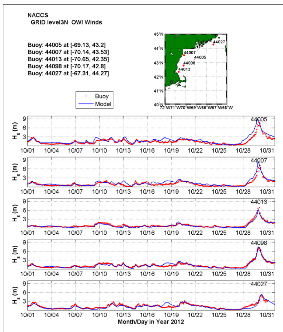
Figure 5-8. Evaluation of WAM Level3N, northern region results for five wave measurement locations.
