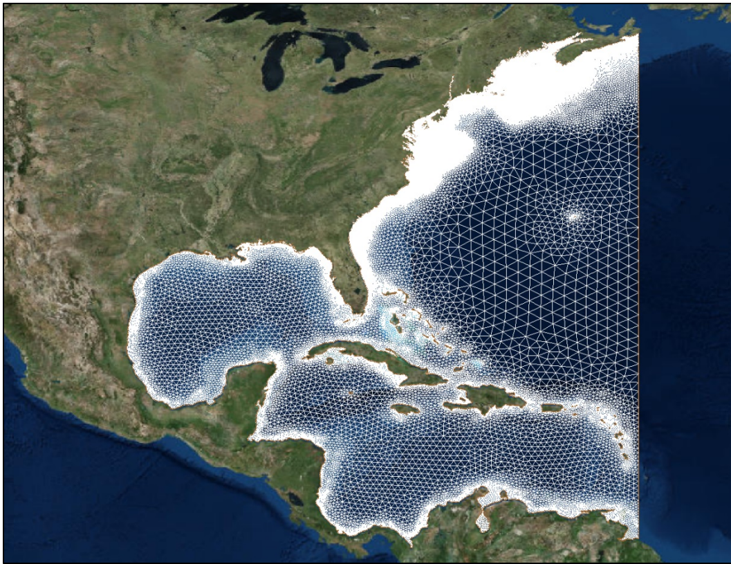
Figure 6-2. ADCIRC mesh for NACCS.
