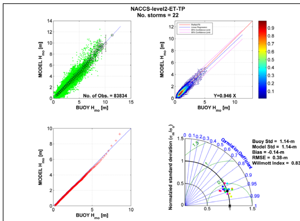
Figure 5-19. Bin average scatter diagram (top left), color contour (top right), Quartile-Quartile plot (lower left) and Taylor diagram (lower right) for WAM Level2 results derived from the extra- and tropical storm set.
