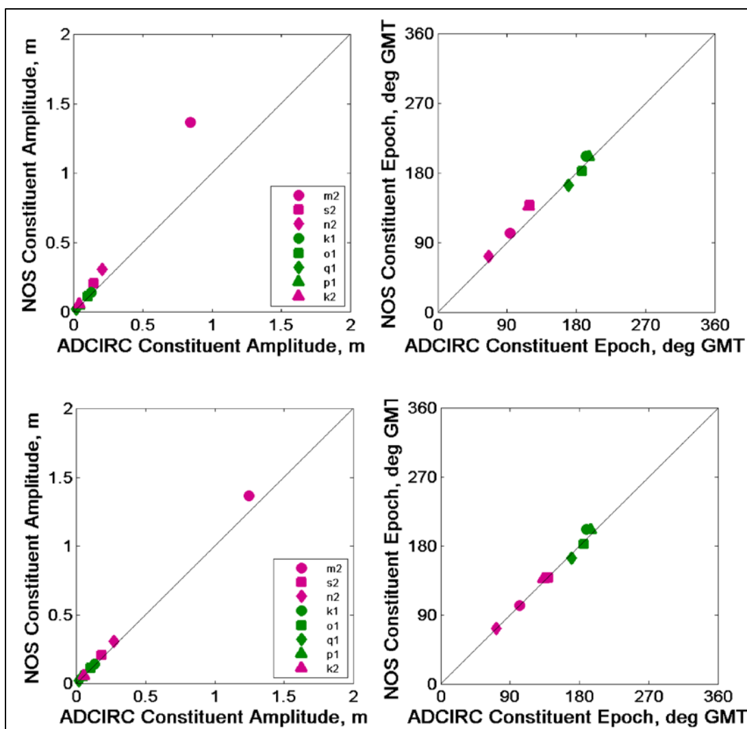
Figure 6-21. Tidal harmonic analysis for Portland, Maine gage top) before and bottom) after Gulf of Maine bathymetric correction.
