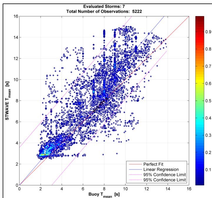
Figure 7-25. Color contour of time paired mean wave period for all validation storms.
