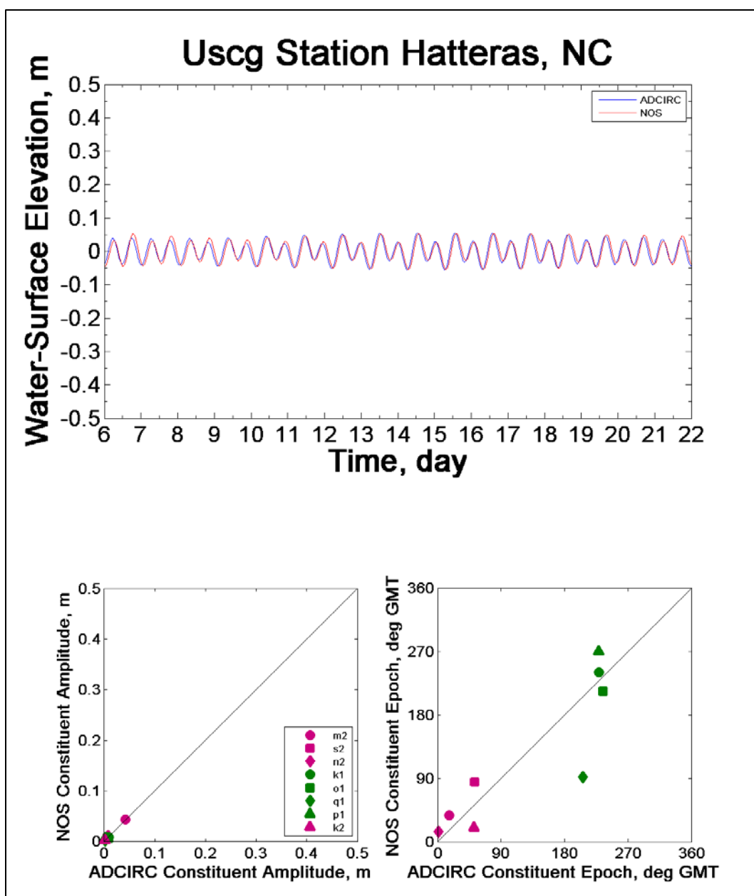
Figure 6-26. Tidal harmonic analysis for the US Coast Guard Station, Hatteras, NC.
