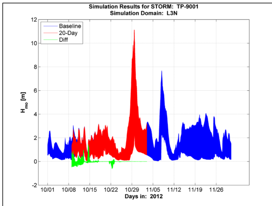
Figure 5-15. Time plot envelope of 165 special output locations for 20-day pad SuperStorm Sandy.
