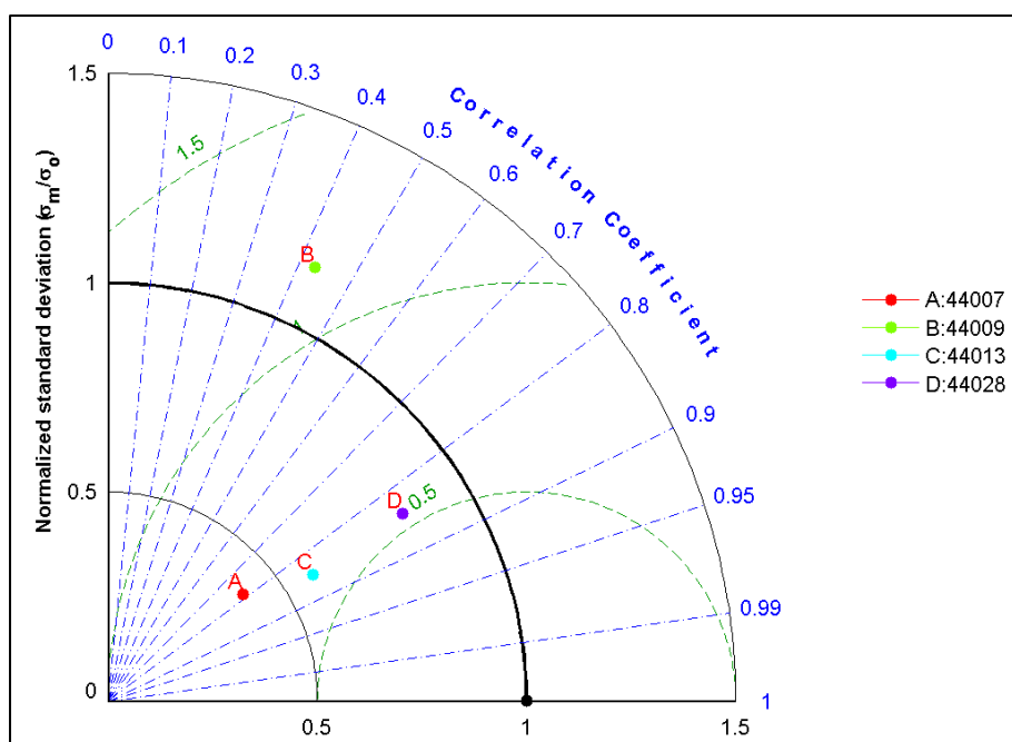
Figure 7-16. Taylor diagram for ET073.
