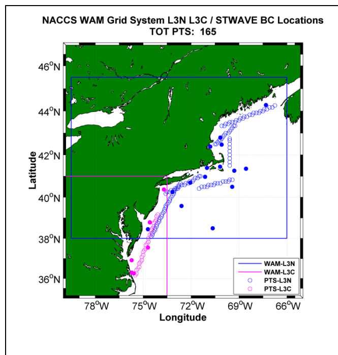
Figure 5-7. STWAVE boundary condition save points (open circles), buoy sites (solid points). Initialization analyses use both STWAVE boundary points and measurement sites.
