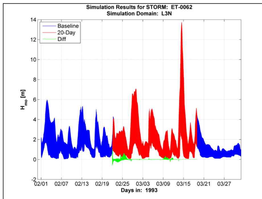
Figure 5-11. Time plot envelope of 165 special output locations for 20-day pad, Storm of the Century.
