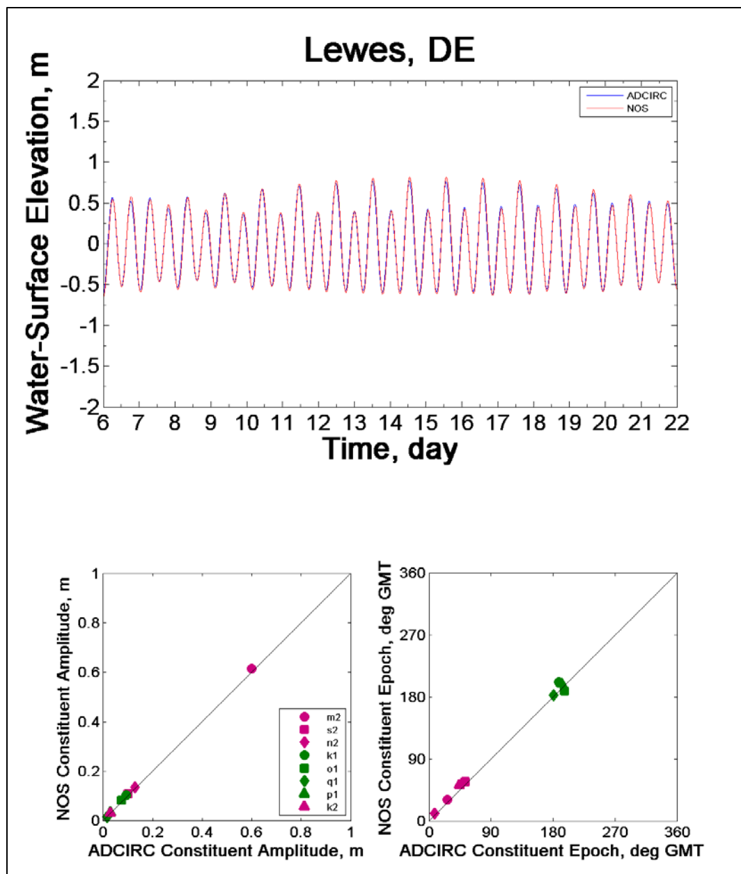
Figure 6-25. Tidal harmonic analysis for Lewes, Delaware.
