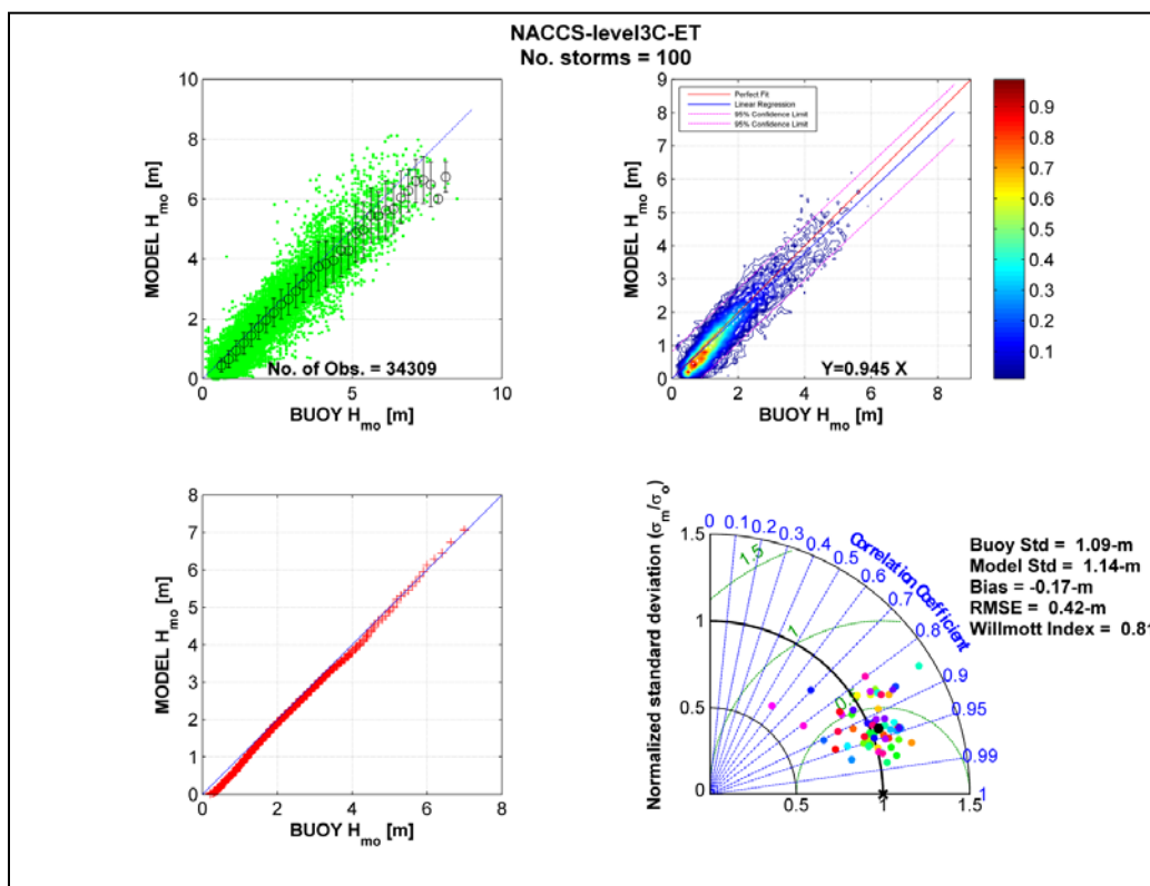
Figure 5-28. Bin average scatter diagram (top left), color contour (top right), Quartile-Quartile plot (lower left) and Taylor diagram (lower right) for WAM Level3c results derived from the 100 extreme extratropical storm events.
