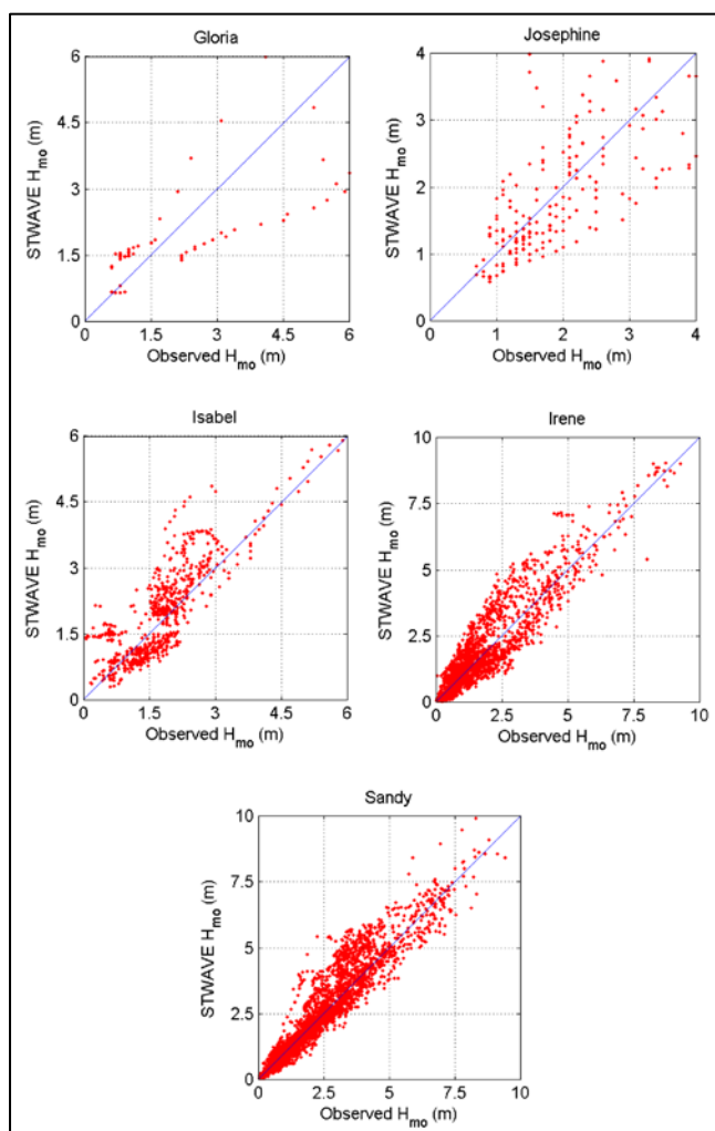
Figure 7-23. Scatter plots of validation tropical storms.
