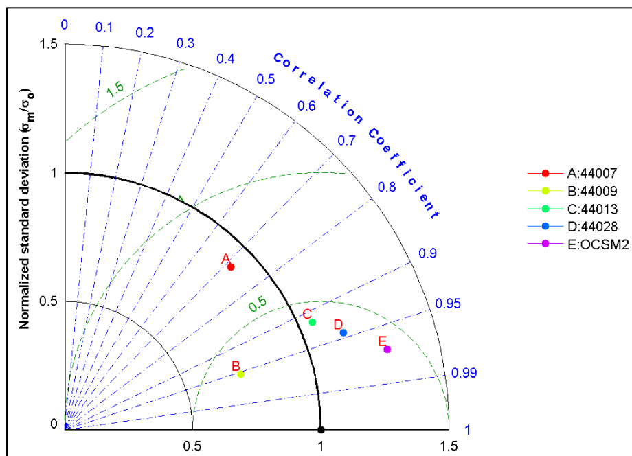
Figure 7-15. Taylor diagram for ET070.
