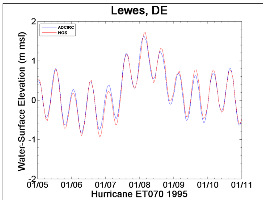
Figure 6-36. ET070 time series comparison at Lewes, Delaware.
