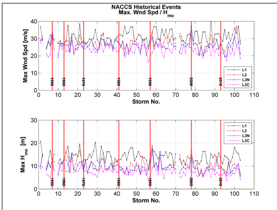
Figure 5-23. Maximum wind speed and H_{mo} estimates for 100 extratropical historical storm simulations. Decades are indicated by the red vertical lines.
