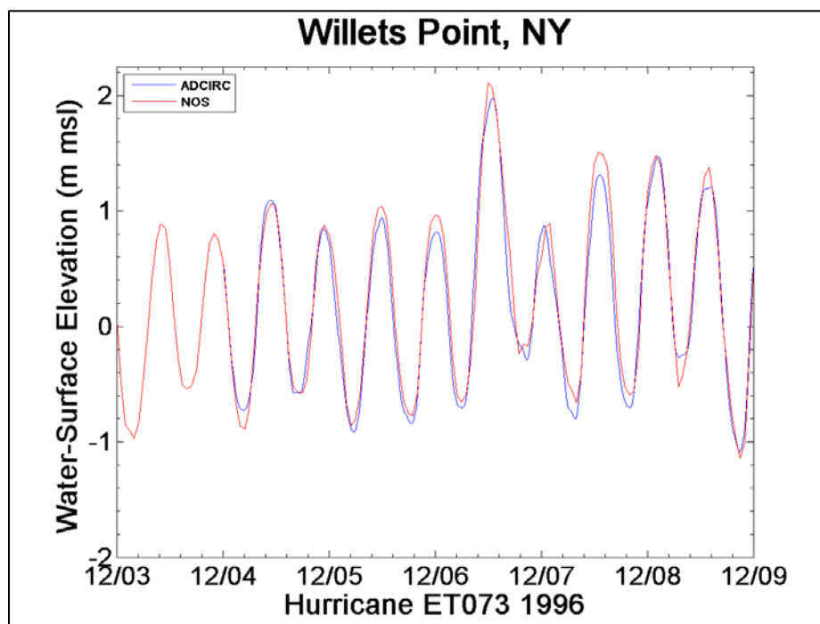
Figure 6-37. ET073 time series comparison at Willets Point, New York.
