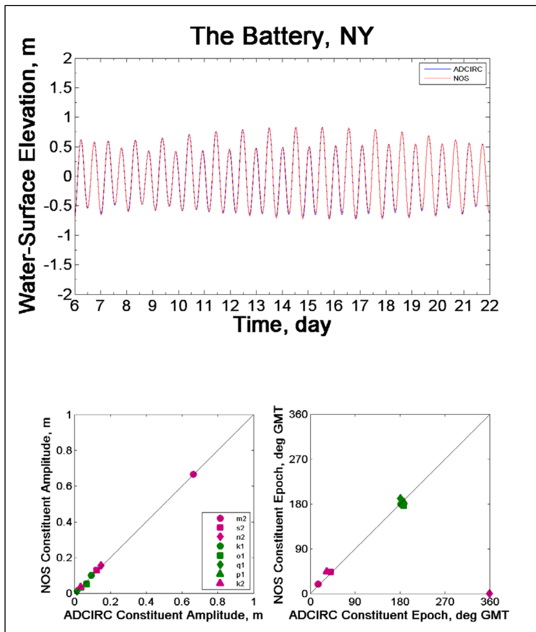
Figure 6-23. Tidal harmonic analysis for The Battery, New York.
