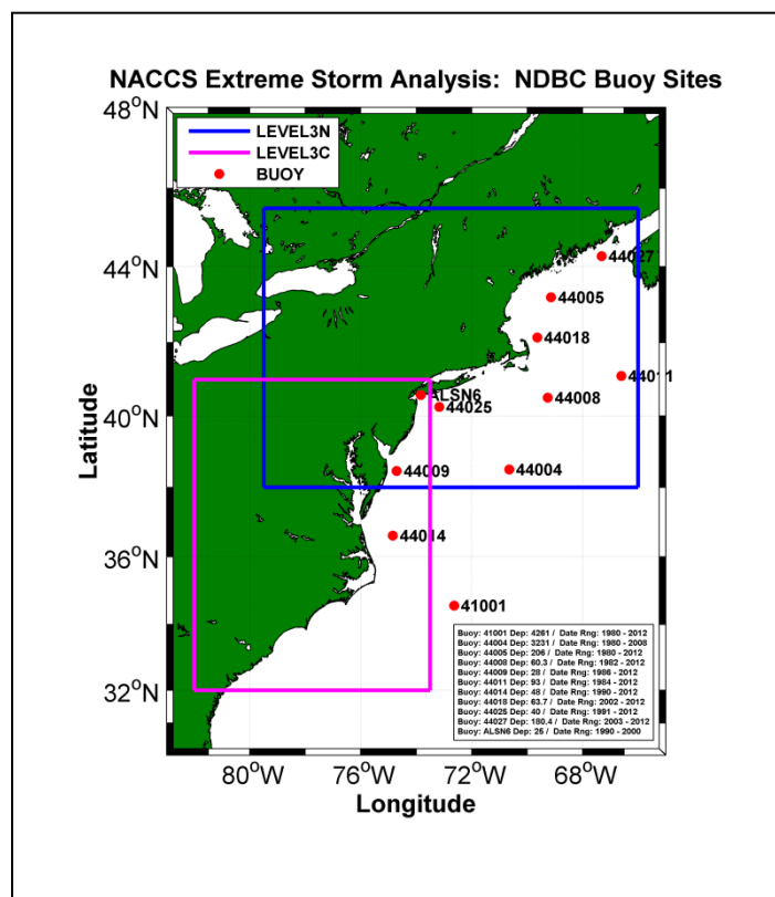
Figure 5-1. Offshore wave model Regional and Sub-region domains, and NOAA National Data Buoy Center sites used for extreme wave storm analysis.
