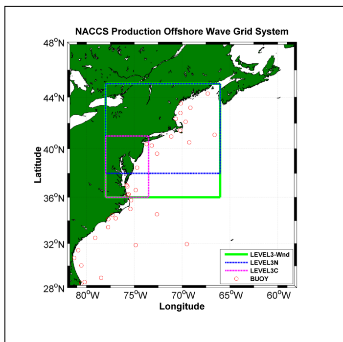
Figure 5-22. WAM multi-level grid system used in NACCS Production. Note Level 2 covers the entire domain illustrated, (compared to Figure 5-5 displaying evaluation test grid systems).
