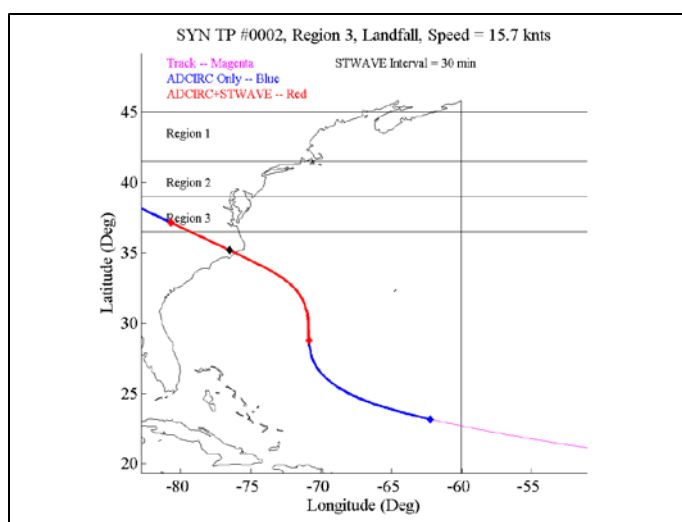
Figure 8-7. Synthetic tropical storm number 2's track (a land-falling storm) and indicators for ADCIRC only (blue) computations and ADCIRC+STWAVE (red) computations along the track.
