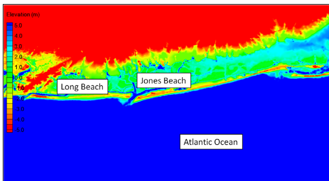
Figure 6-5. ADCIRC mesh topography/bathymetry for a portion of Long Island, New York before 2012 LIDAR update.
