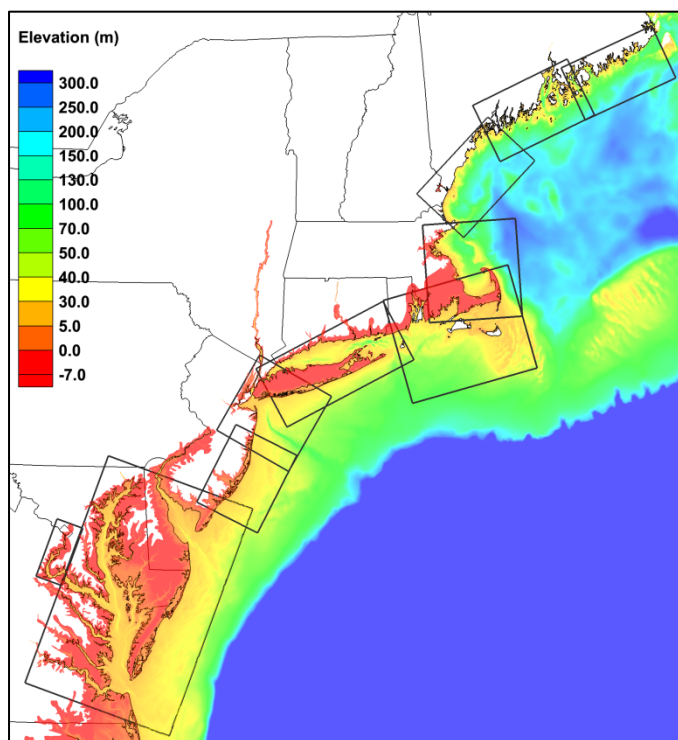
Figure 7-1. STWAVE grid domains.
